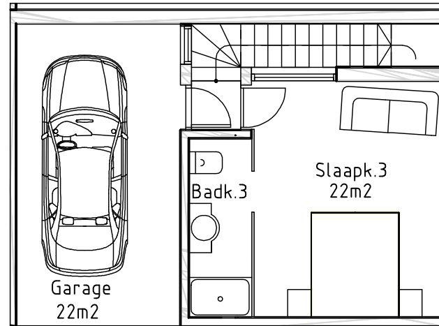
Verdieping -1
